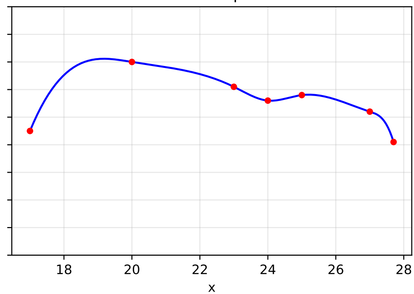
Curva 2: Spline
