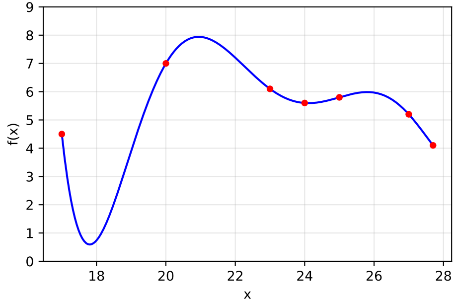
Curva 2: Vandermonde
